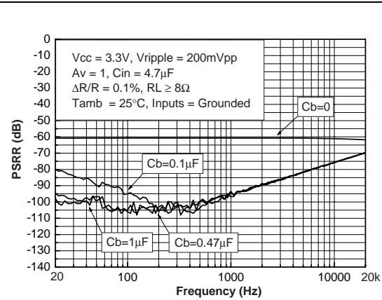
Figure 71. PSRR vs. frequency (worst case conditions)
