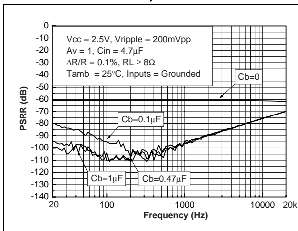
Figure 72. PSRR vs. frequency (worst case conditions)
